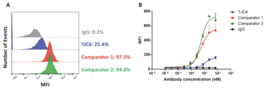
Figure: Binding of CD47 monoclonal antibodies to RBCs. (A) Representative graph of the staining of human RBCs with CD47 monoclonal antibodies or control IgG (1 \mu g/ml); (B) Dose dependent binding of CD47 monoclonal antibodies with human RBCs from different healthy donors ( n = 3 ). MFI: mean fluorescence intensity.
